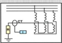
Examples of providing artificial neutral point if it is impossible to reach the neutral point of the source or the connection is delta.
